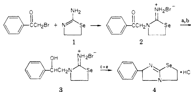
Scheme I a
